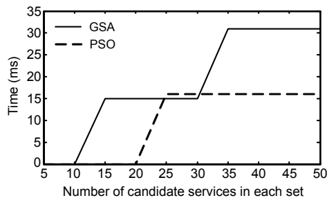
Fig. 14 Change of time with increase in the number of candidate services, with n=5 , m=6 , \text{num}=10 , and T=80
