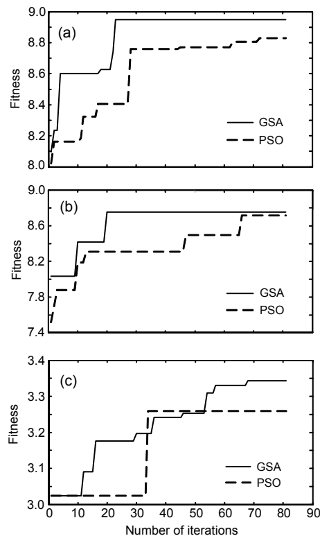
Fig. 7 Fitness change with increase in the number of algorithm repetitions
