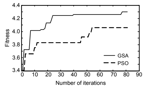
Fig. 11 Fitness change with increase in the number of algorithm repetitions, with n=10 , l=12 , m=6 , \text{num}=4 , and T=80
