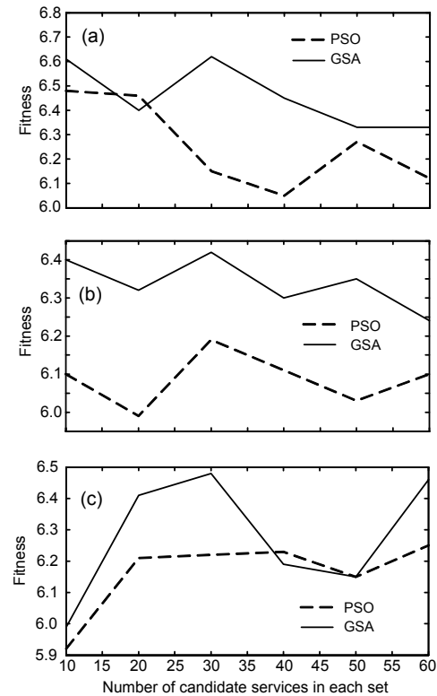
Fig. 8 Fitness change with increase in the number of candidate services
