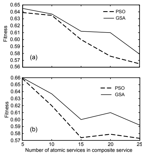
Fig. 9 Fitness change with increase in the number of atomic services
