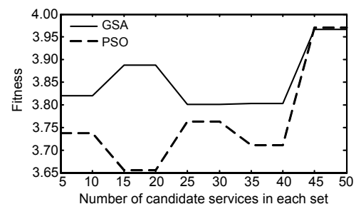
Fig. 12 Fitness change with increase in the number of candidate services, with n=10 , m=6 , \text{num}=10 , and T=80
