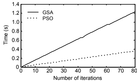
Fig. 13 Change of time with increase in the number of algorithm repetitions, with n=10 , m=6 , \text{num}=10 , and l=10
